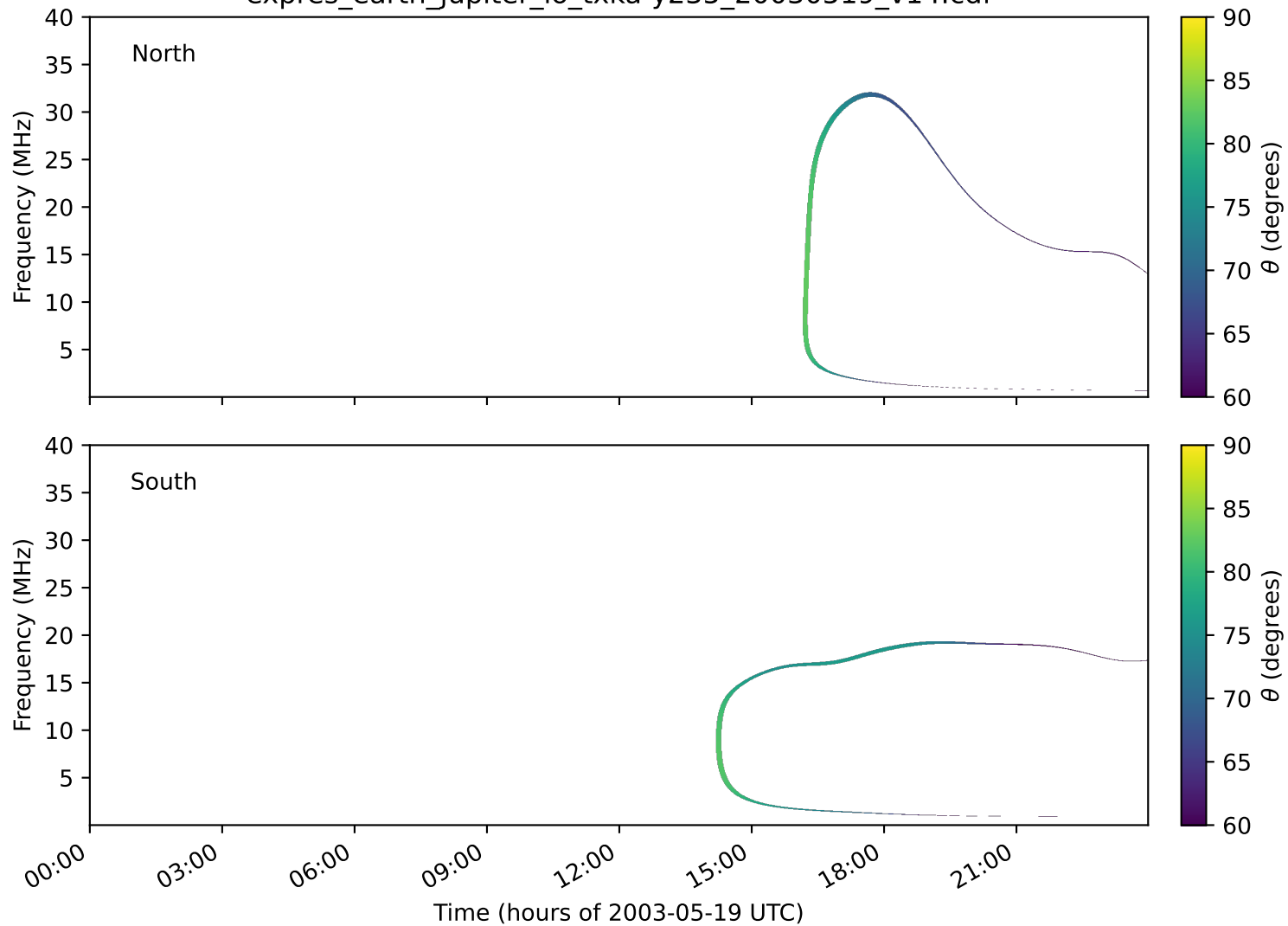
expres_earth_jupiter_io_txka-y235_20030519_v14.cdf
