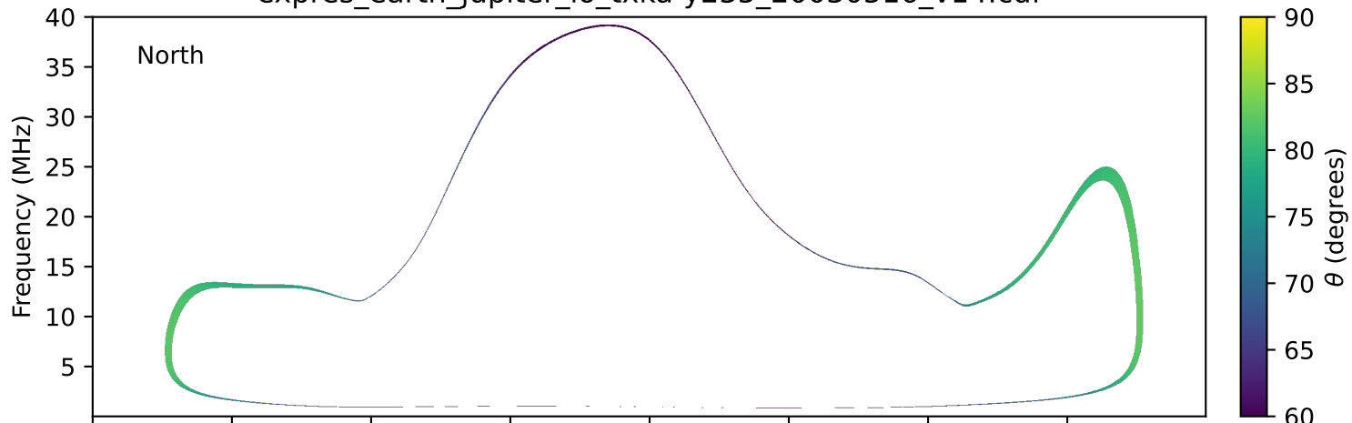
expres_earth_jupiter_io_txka-y235_20030516_v14.cdf
