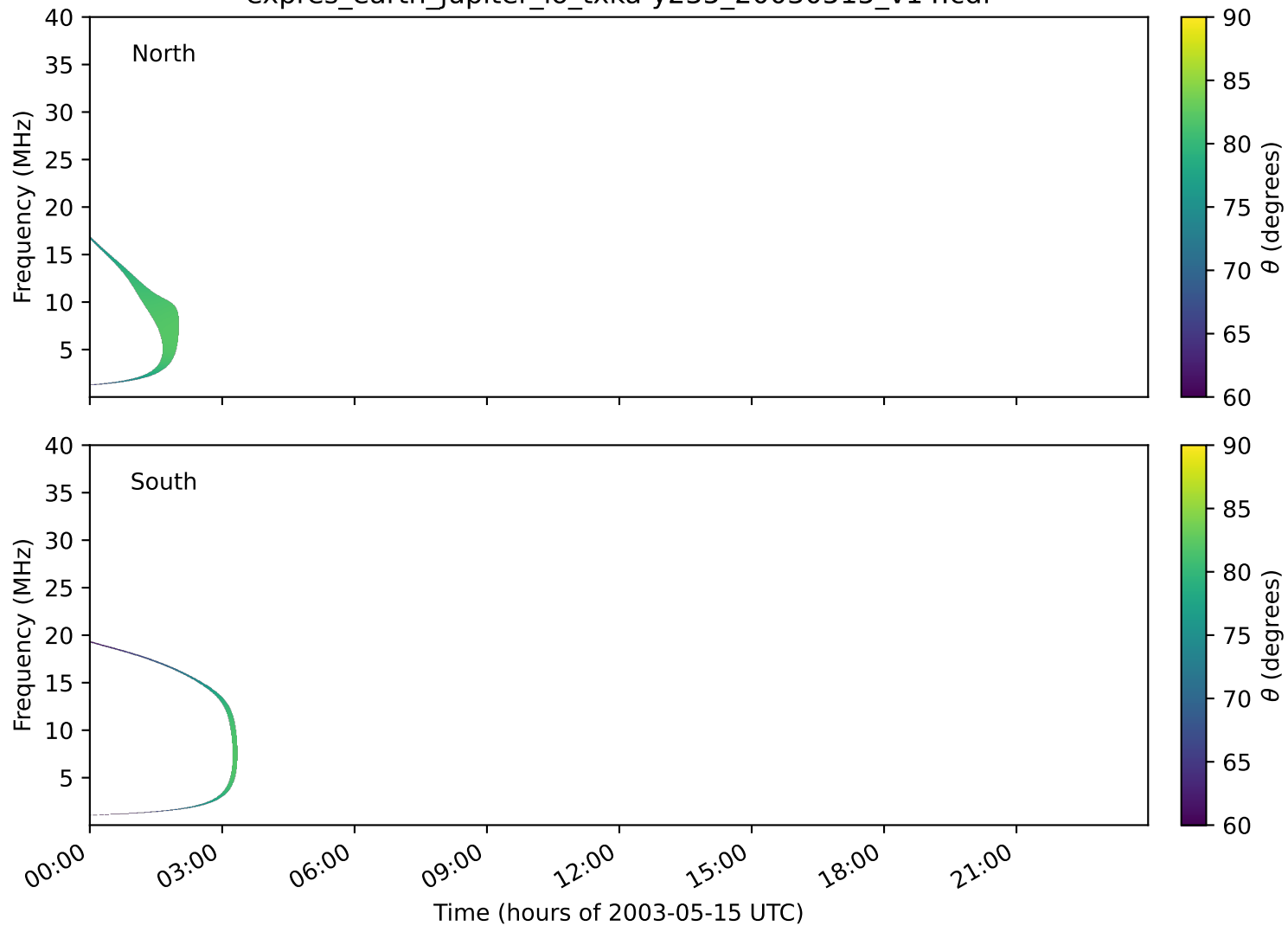
expres_earth_jupiter_io_txka-y235_20030515_v14.cdf
