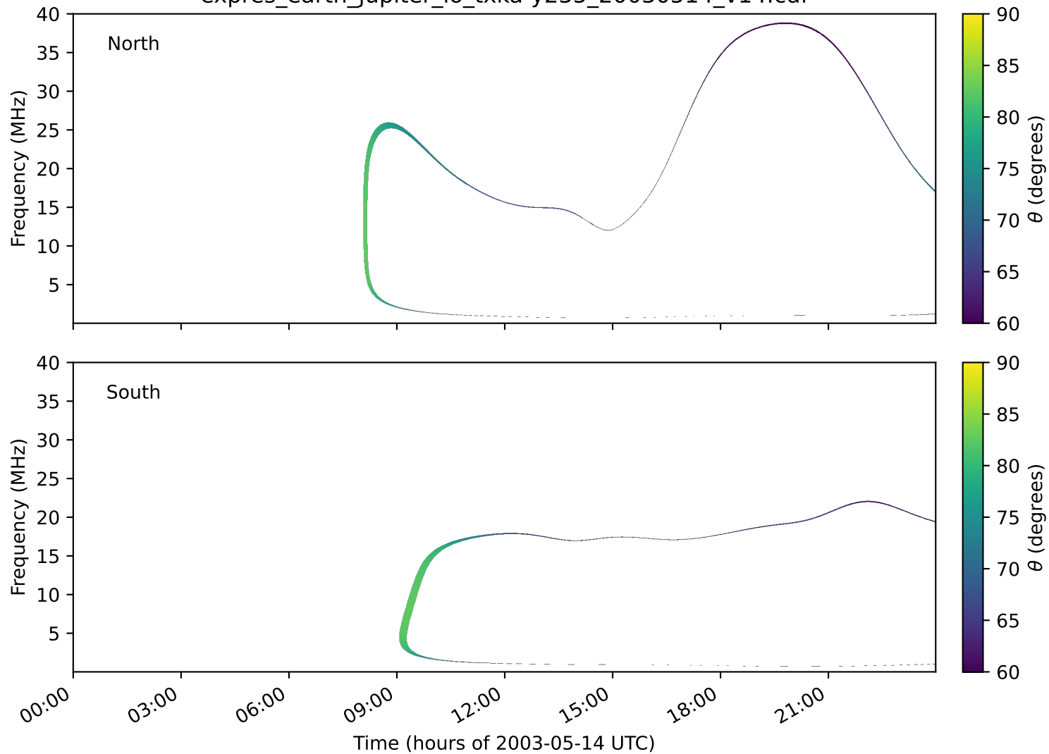
expres_earth_jupiter_io_txka-y235_20030514_v14.cdf
