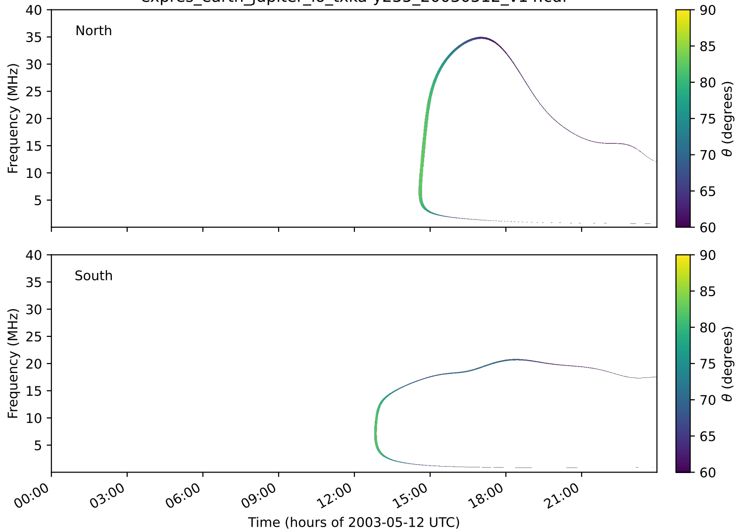
expres_earth_jupiter_io_txka-y235_20030512_v14.cdf
