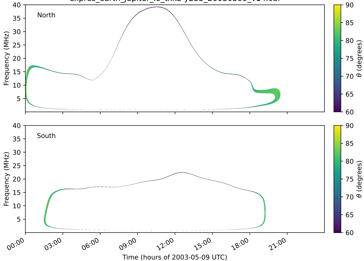
expres_earth_jupiter_io_txka-y235_20030509_v14.cdf
