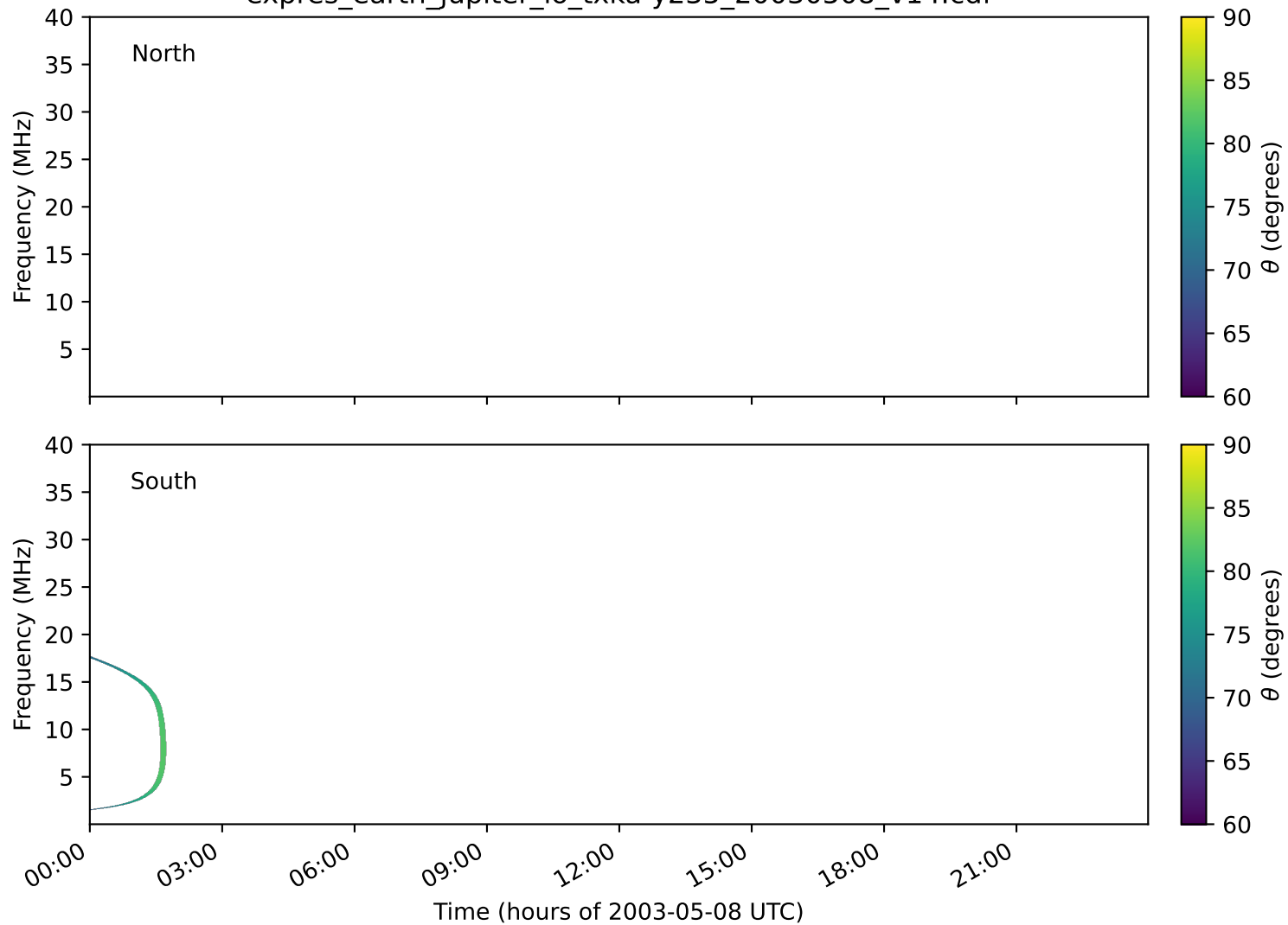
expres_earth_jupiter_io_txka-y235_20030508_v14.cdf
