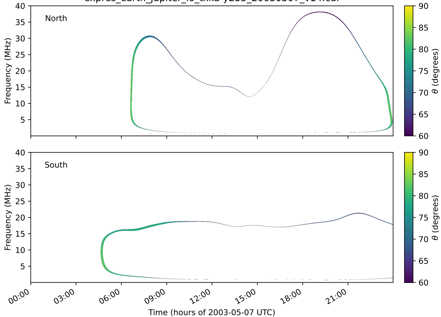
expres_earth_jupiter_io_txka-y235_20030507_v14.cdf
