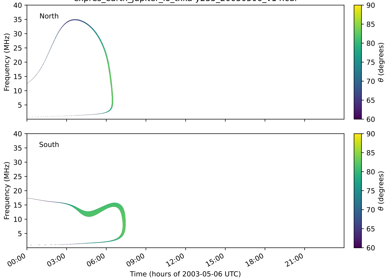
expres_earth_jupiter_io_txka-y235_20030506_v14.cdf
