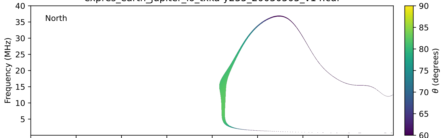
expres_earth_jupiter_io_txka-y235_20030505_v14.cdf
