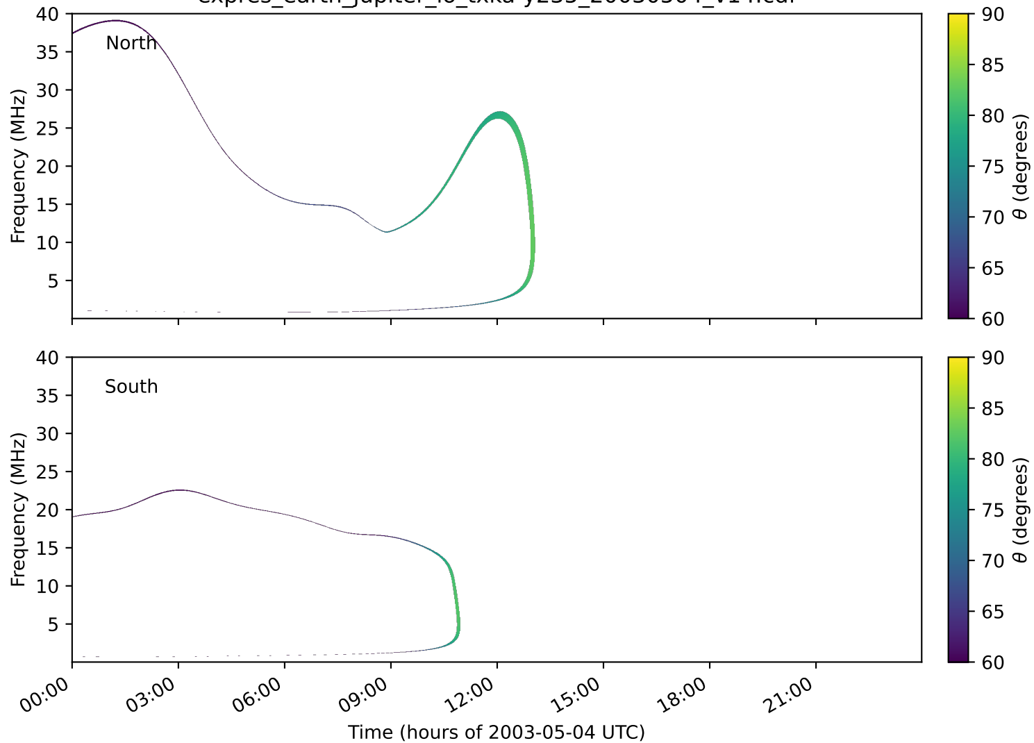
expres_earth_jupiter_io_txka-y235_20030504_v14.cdf
