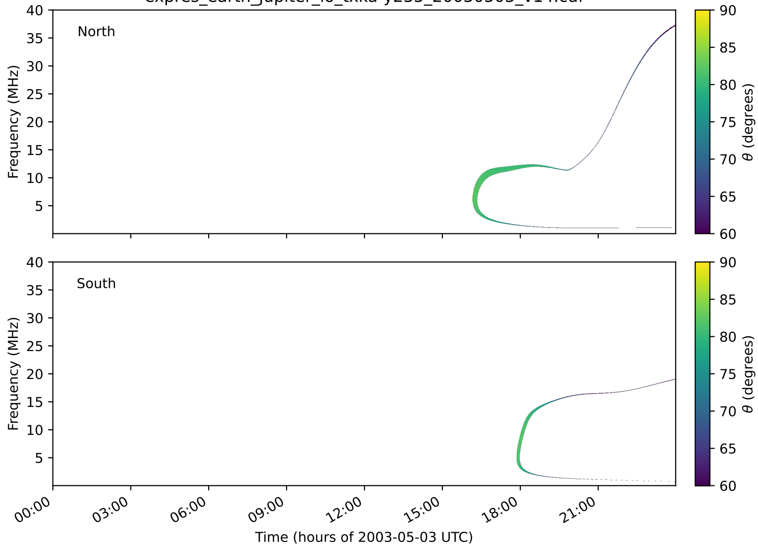
expres_earth_jupiter_io_txka-y235_20030503_v14.cdf
