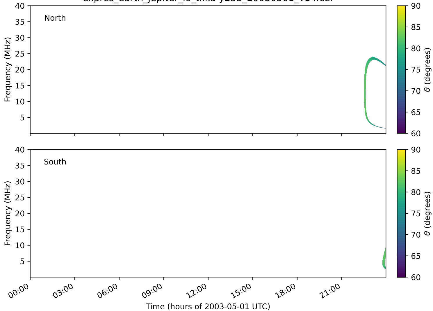
expres_earth_jupiter_io_txka-y235_20030501_v14.cdf
