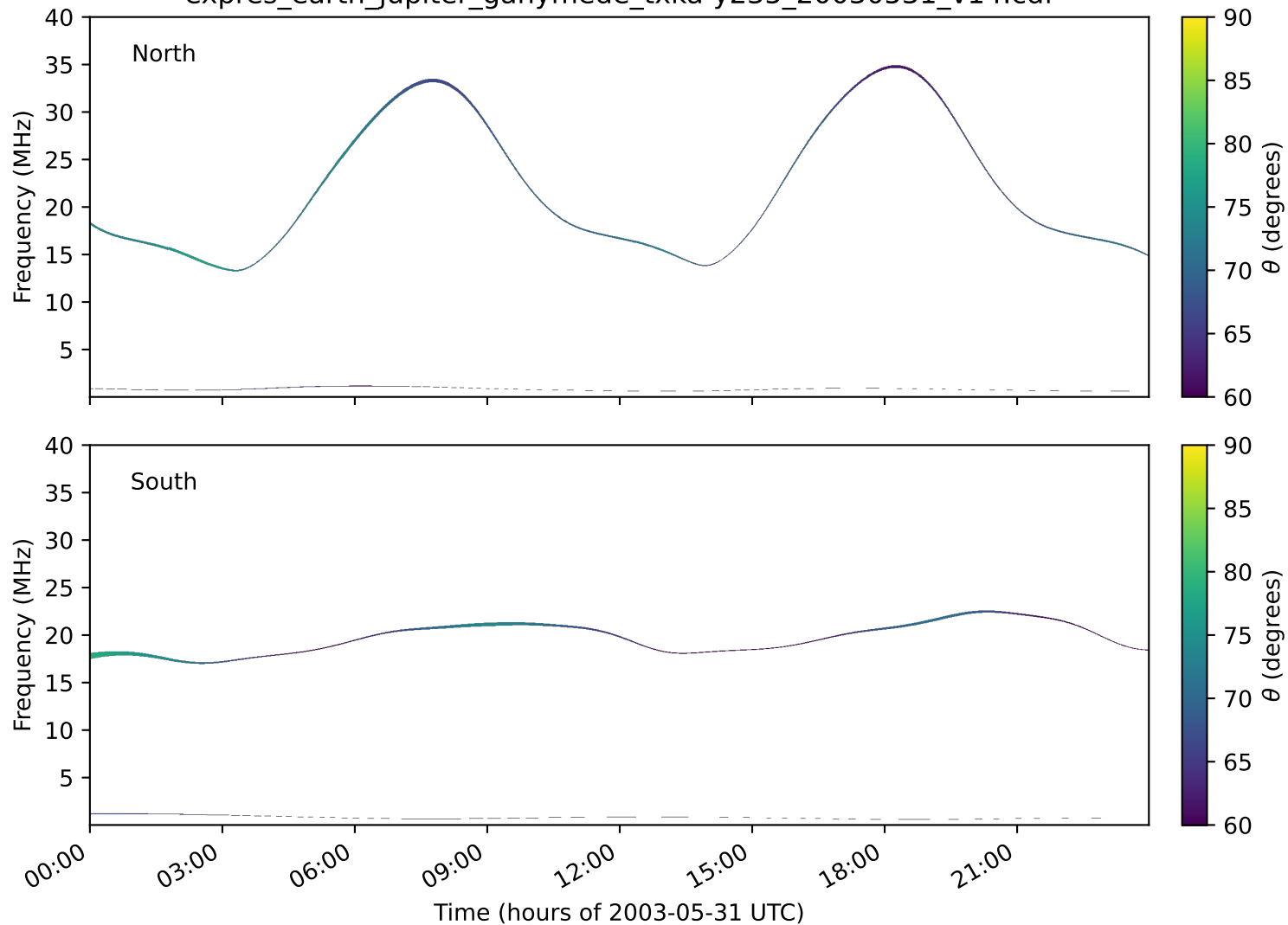
expres_earth_jupiter_ganymede_txka-y235_20030531_v14.cdf
