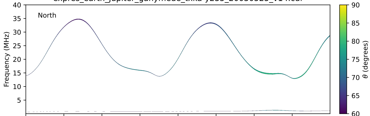
expres_earth_jupiter_ganymede_txka-y235_20030525_v14.cdf
