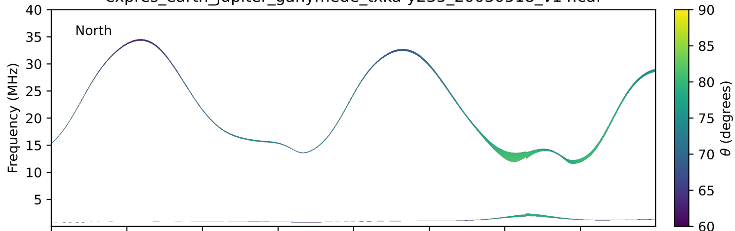
expres_earth_jupiter_ganymede_txka-y235_20030518_v14.cdf
