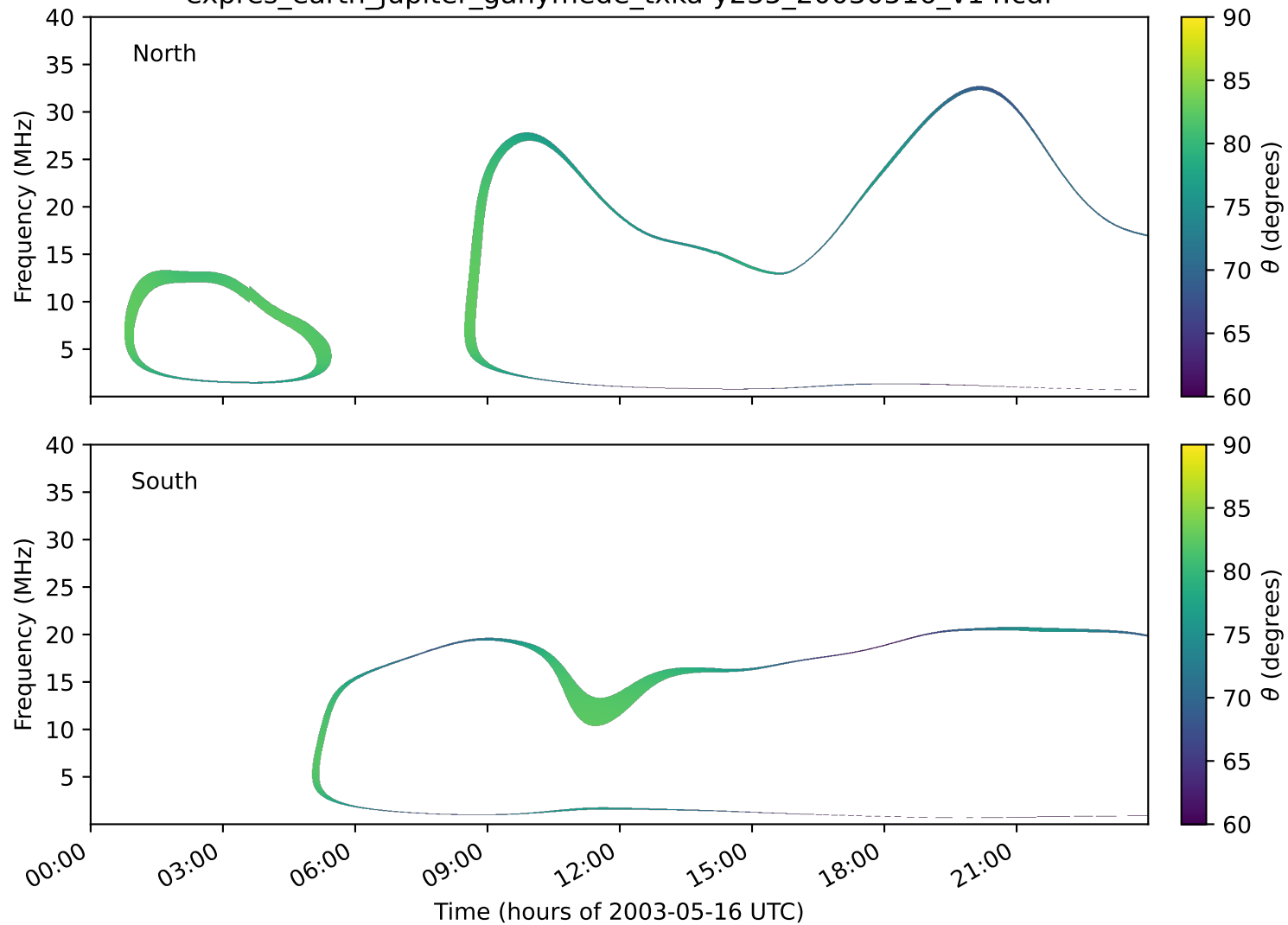
expres_earth_jupiter_ganymede_txka-y235_20030516_v14.cdf
