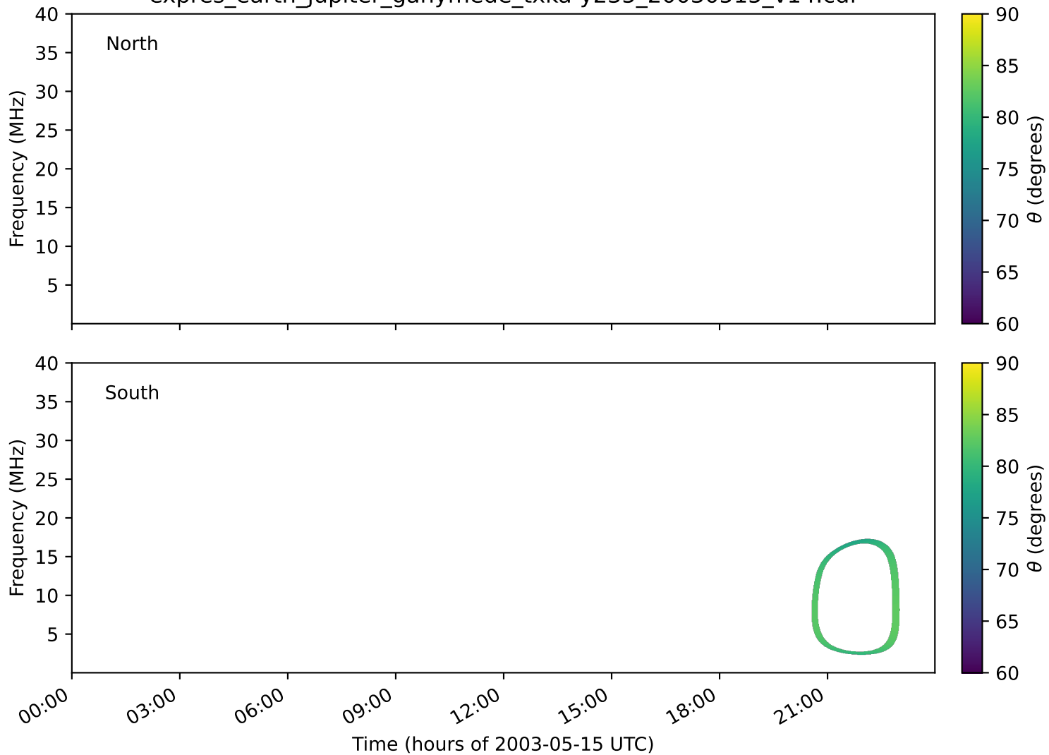
expres_earth_jupiter_ganymede_txka-y235_20030515_v14.cdf
