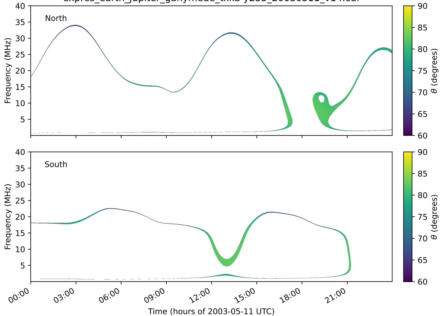
expres_earth_jupiter_ganymede_txka-y235_20030511_v14.cdf
