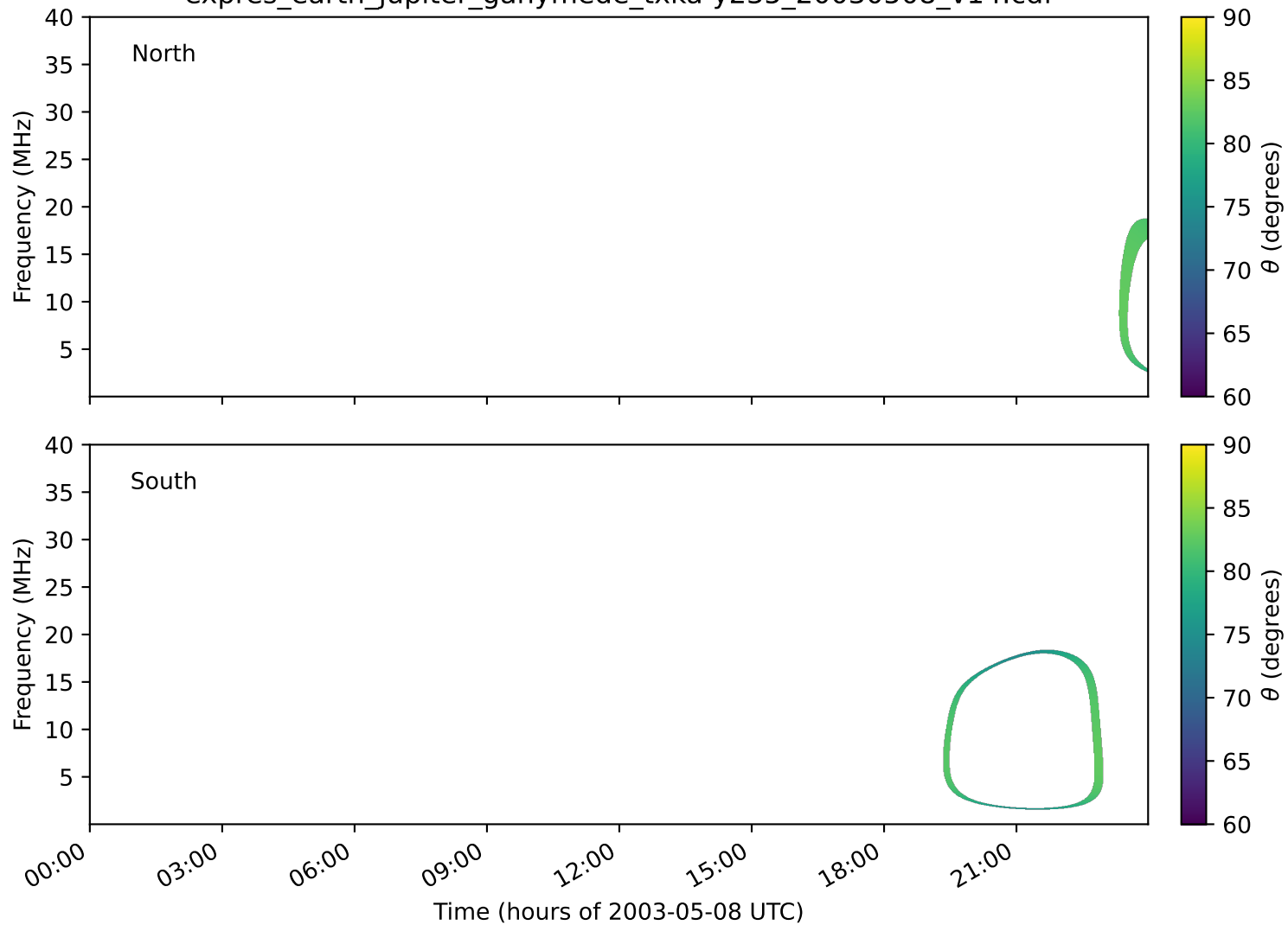
expres_earth_jupiter_ganymede_txka-y235_20030508_v14.cdf
