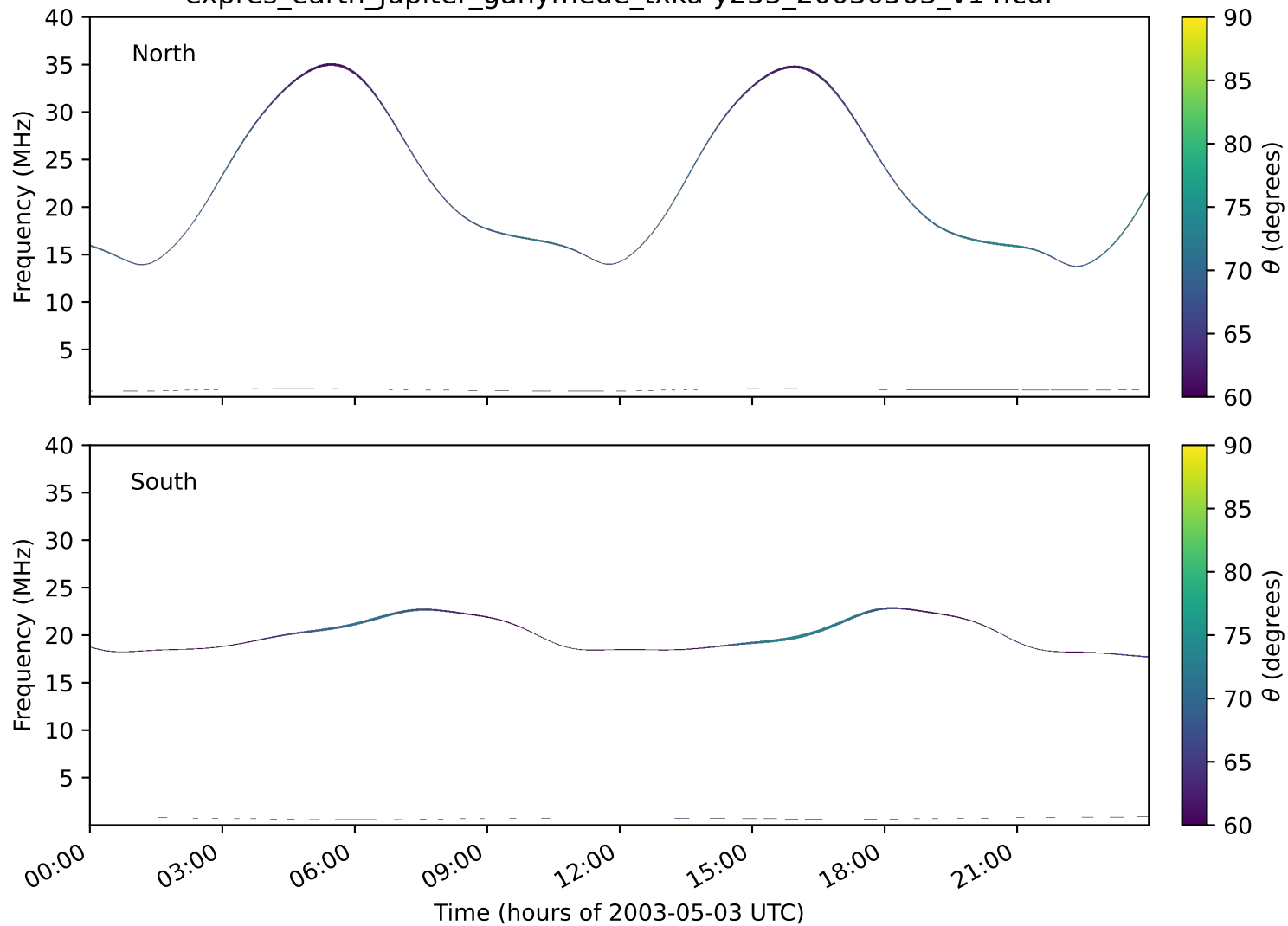
expres_earth_jupiter_ganymede_txka-y235_20030503_v14.cdf
