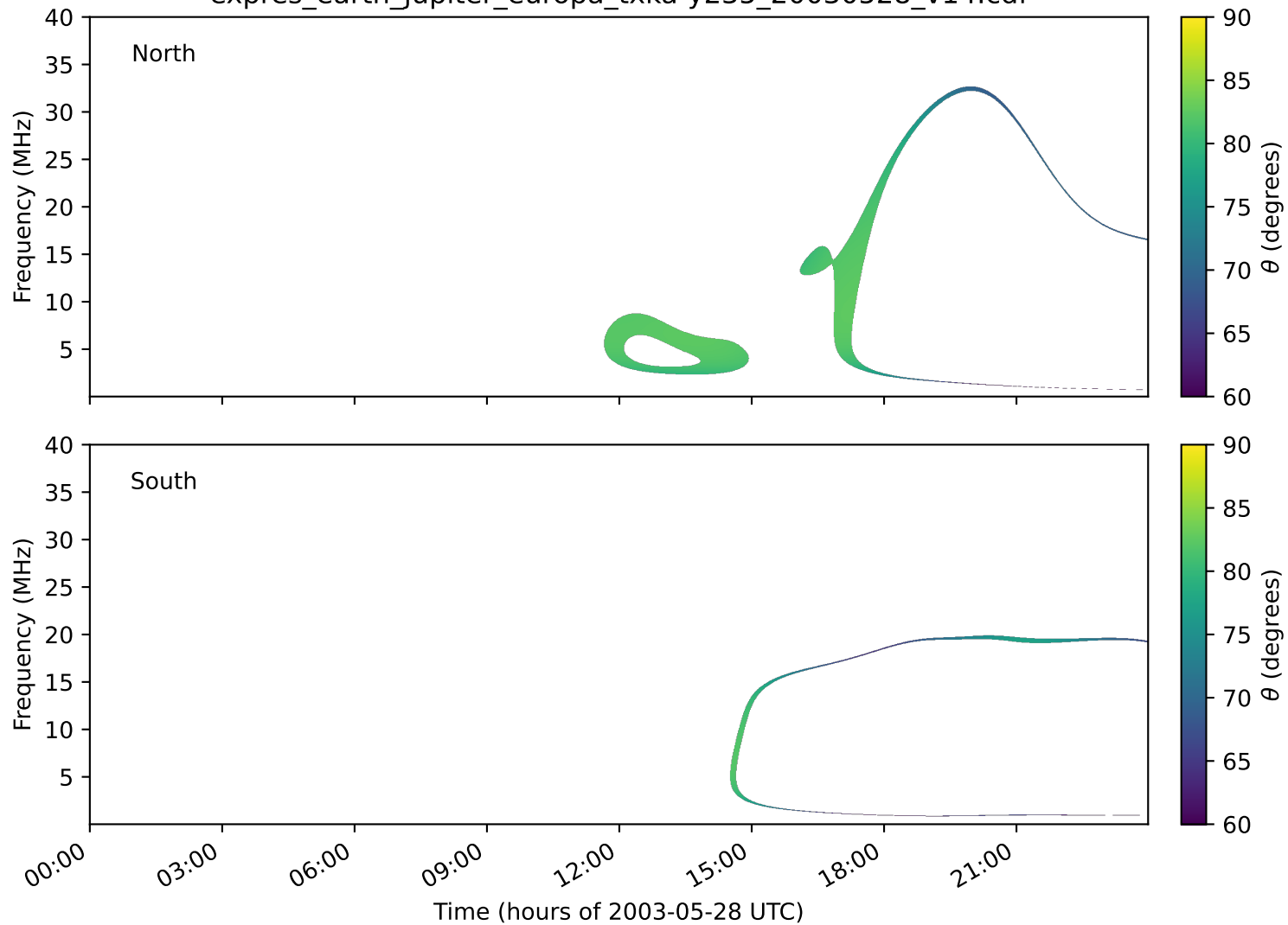
expres_earth_jupiter_europa_txka-y235_20030528_v14.cdf
