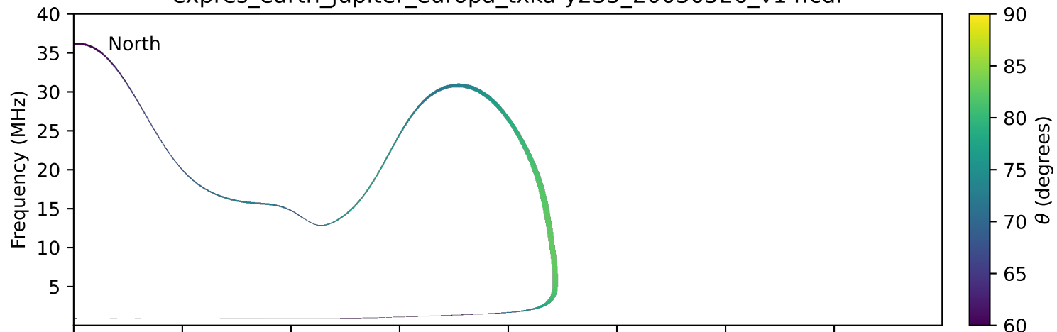
expres_earth_jupiter_europa_txka-y235_20030526_v14.cdf
