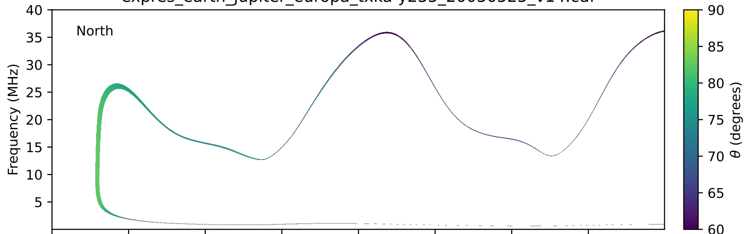
expres_earth_jupiter_europa_txka-y235_20030525_v14.cdf
