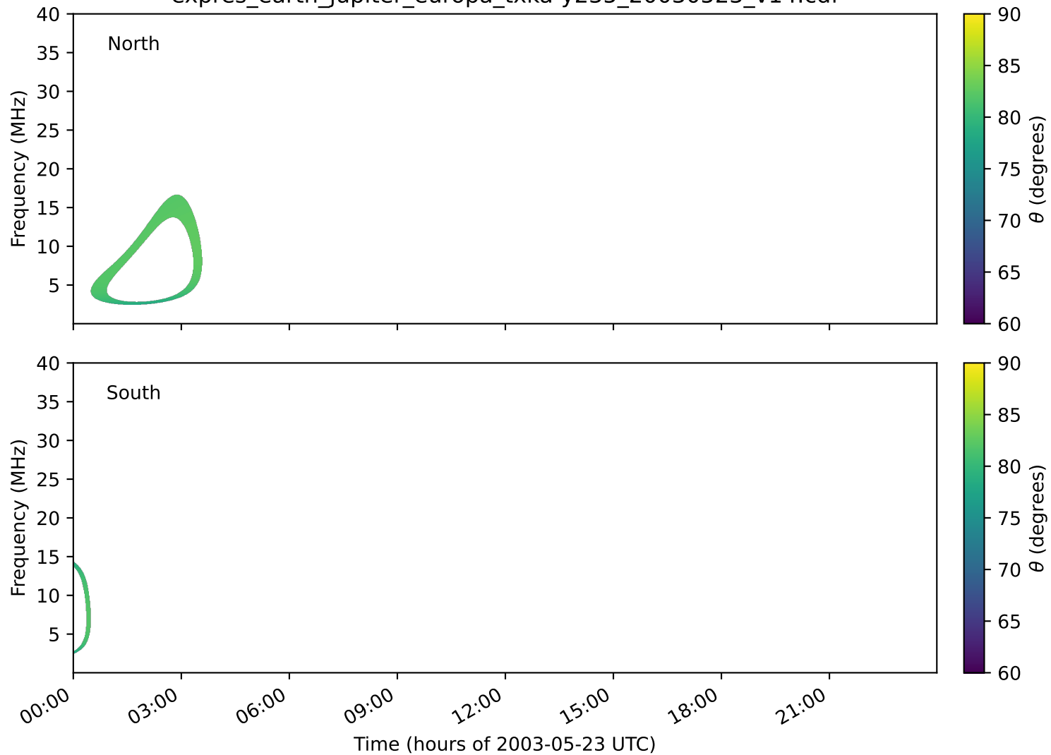
expres_earth_jupiter_europa_txka-y235_20030523_v14.cdf
