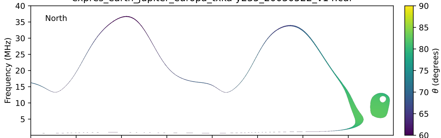
expres_earth_jupiter_europa_txka-y235_20030522_v14.cdf
