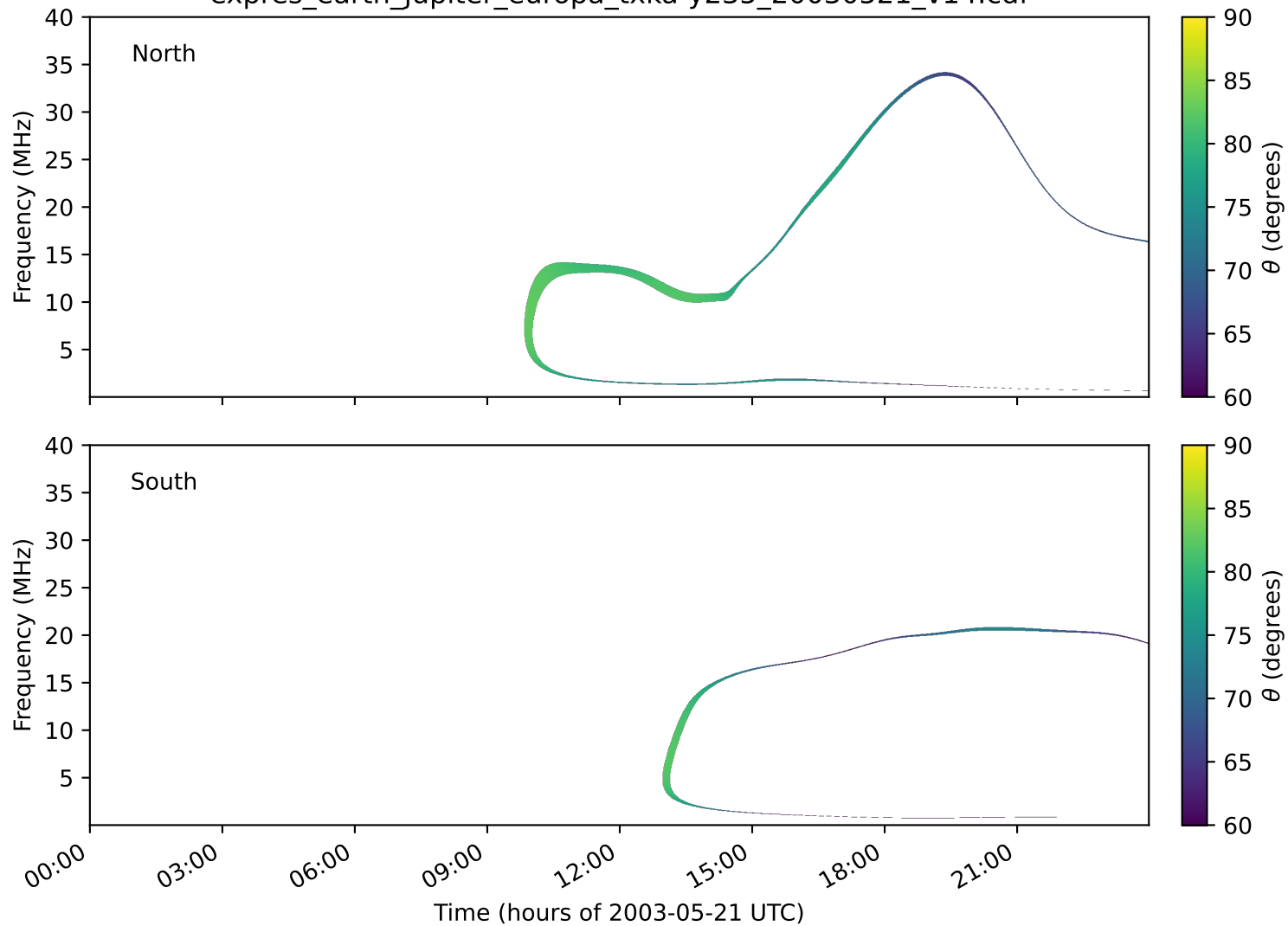
expres_earth_jupiter_europa_txka-y235_20030521_v14.cdf
