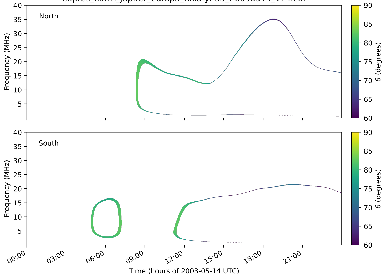
expres_earth_jupiter_europa_txka-y235_20030514_v14.cdf
