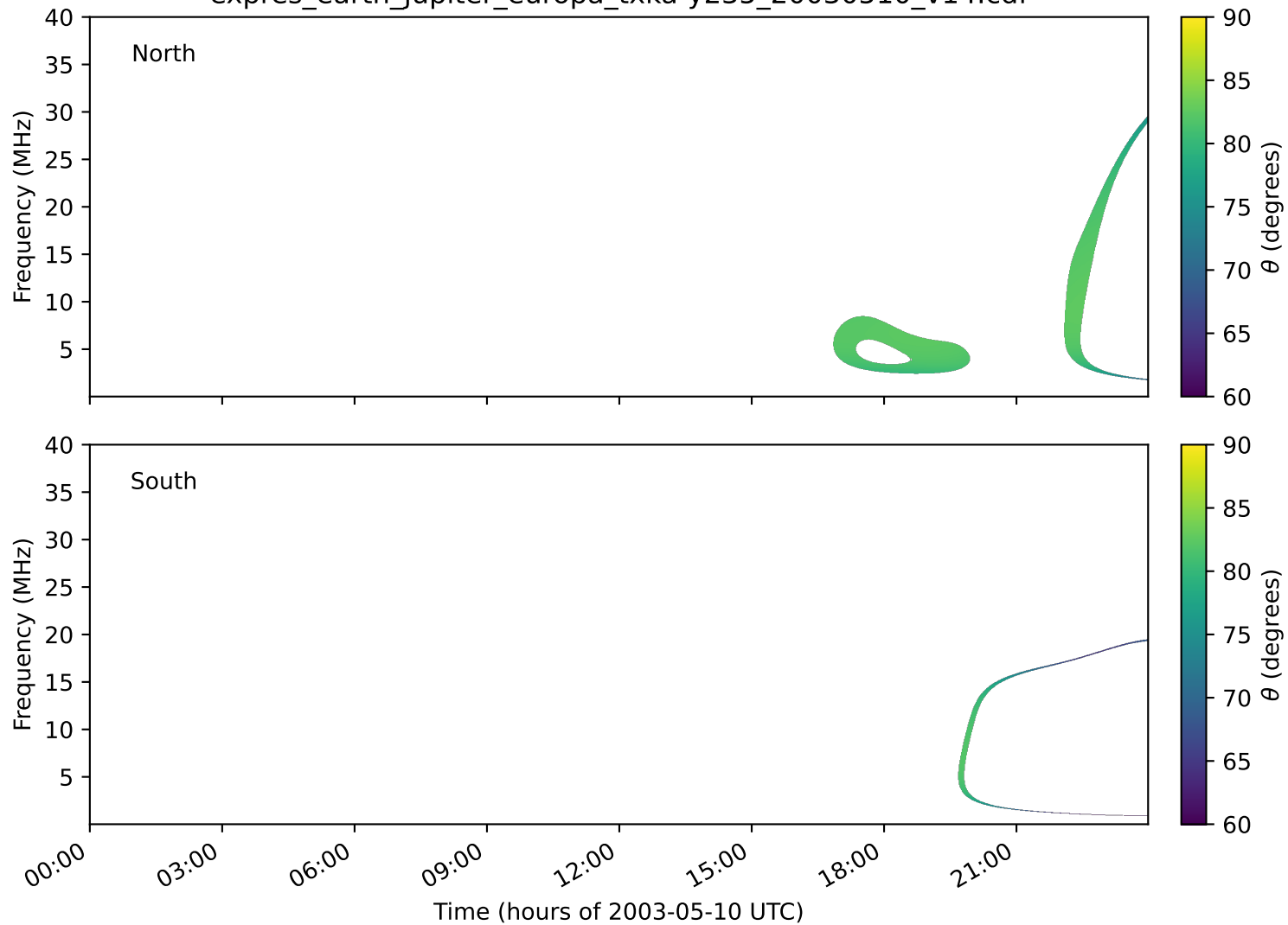
expres_earth_jupiter_europa_txka-y235_20030510_v14.cdf
