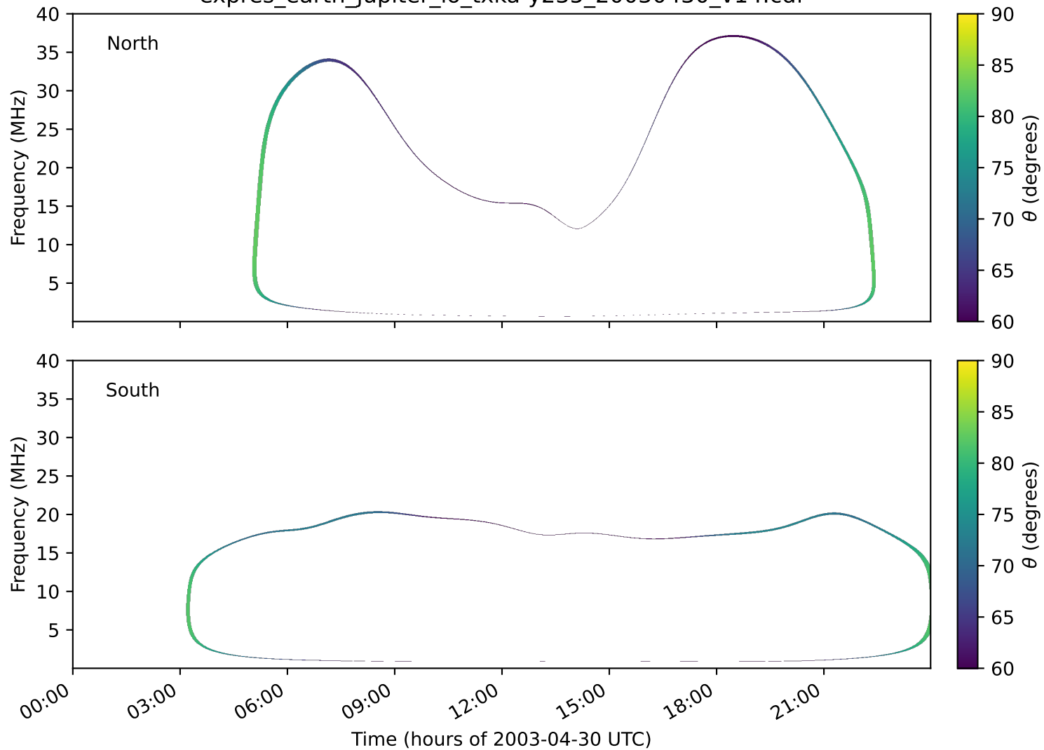
expres_earth_jupiter_io_txka-y235_20030430_v14.cdf
