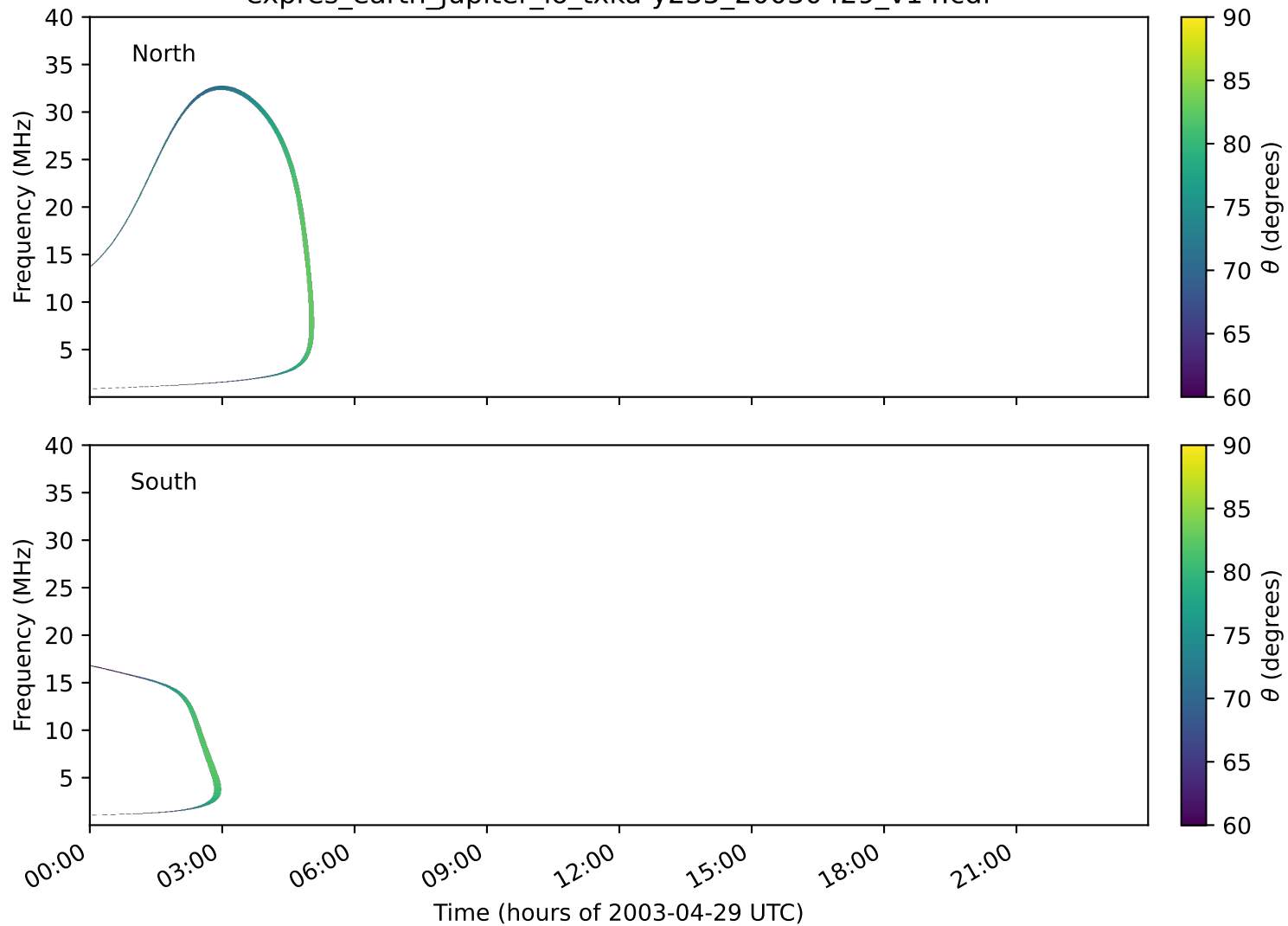
expres_earth_jupiter_io_txka-y235_20030429_v14.cdf
