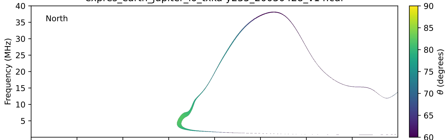
expres_earth_jupiter_io_txka-y235_20030428_v14.cdf
