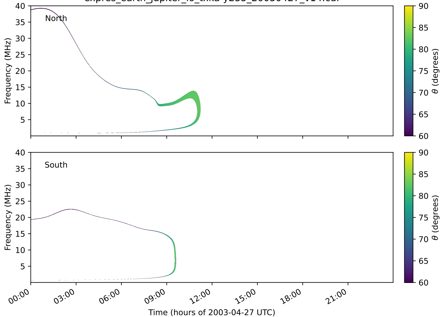
expres_earth_jupiter_io_txka-y235_20030427_v14.cdf
