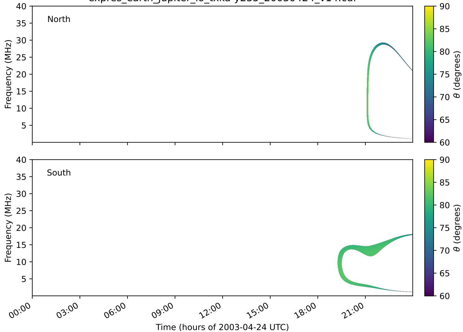
expres_earth_jupiter_io_txka-y235_20030424_v14.cdf
