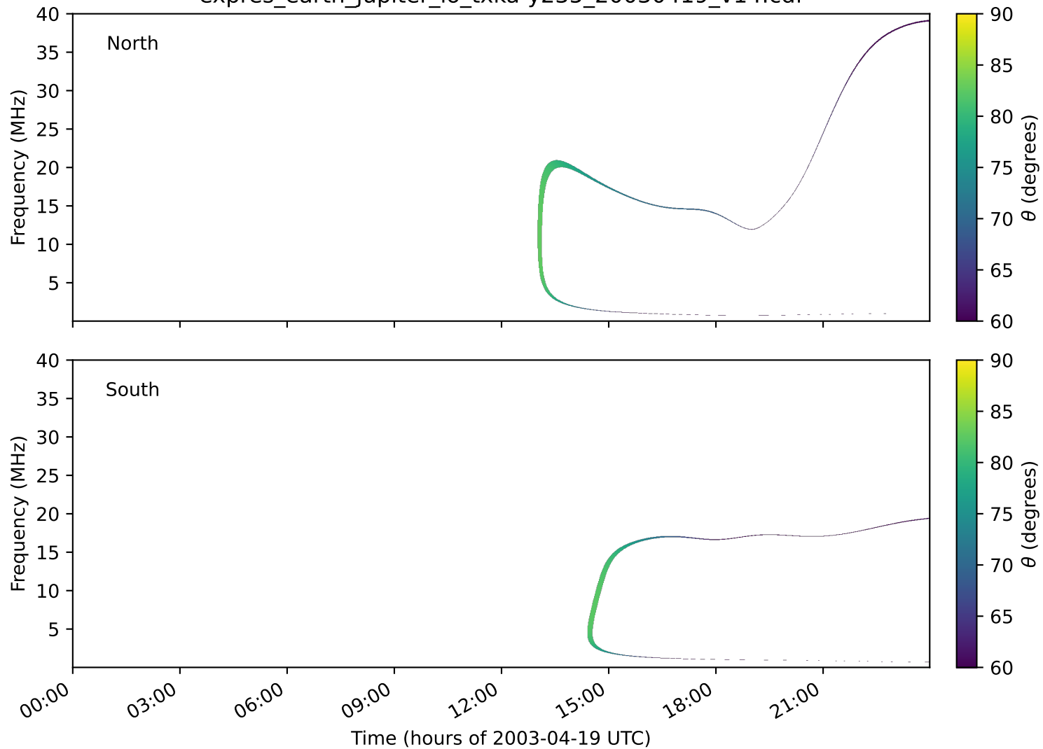
expres_earth_jupiter_io_txka-y235_20030419_v14.cdf
