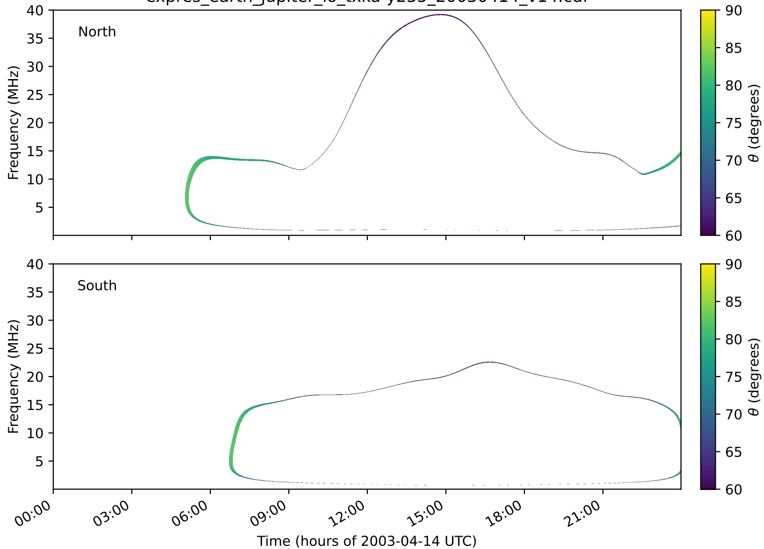
expres_earth_jupiter_io_txka-y235_20030414_v14.cdf
