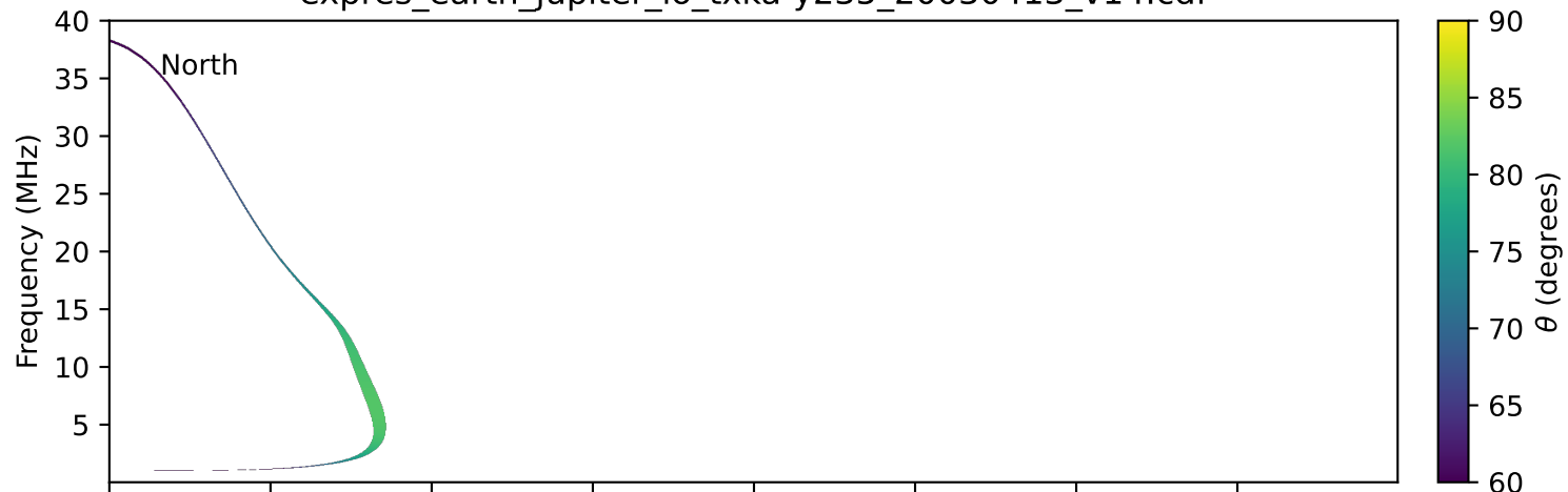
expres_earth_jupiter_io_txka-y235_20030413_v14.cdf
