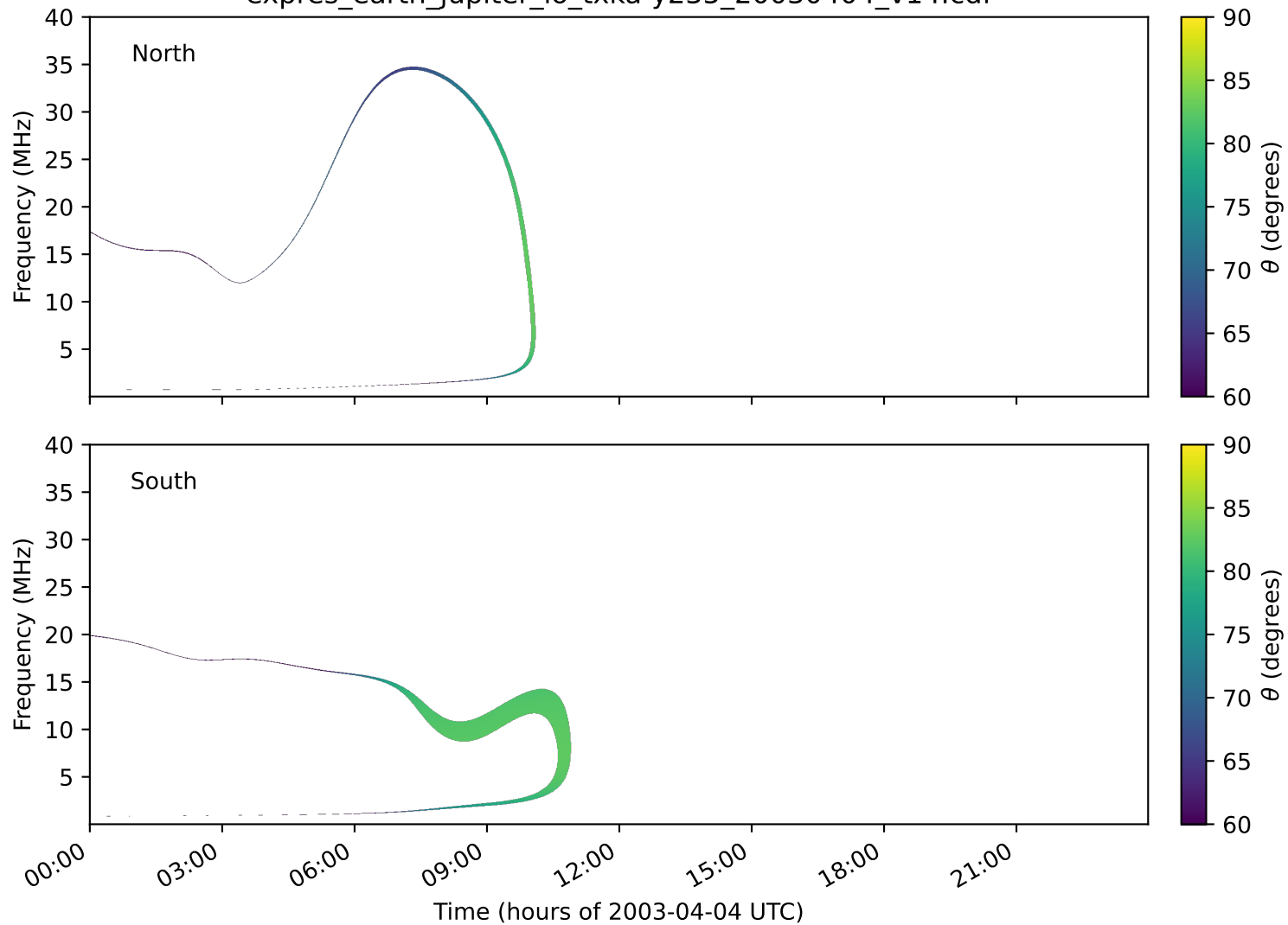
expres_earth_jupiter_io_txka-y235_20030404_v14.cdf
