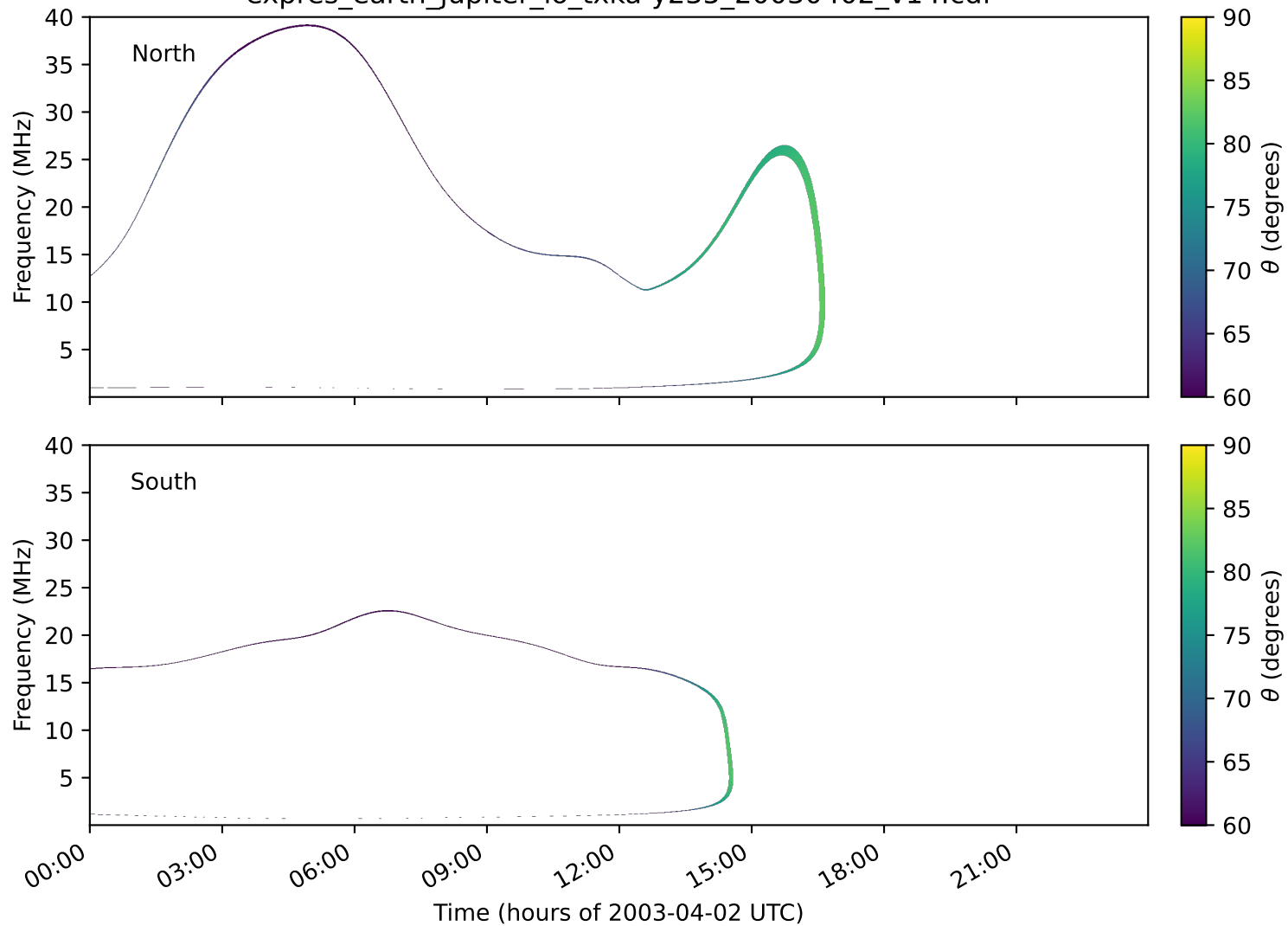
expres_earth_jupiter_io_txka-y235_20030402_v14.cdf
