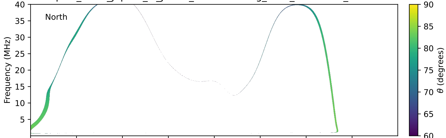
expres_earth_jupiter_io_jrm33_lossc-wid1deg_3kev_20030416_v11.cdf
