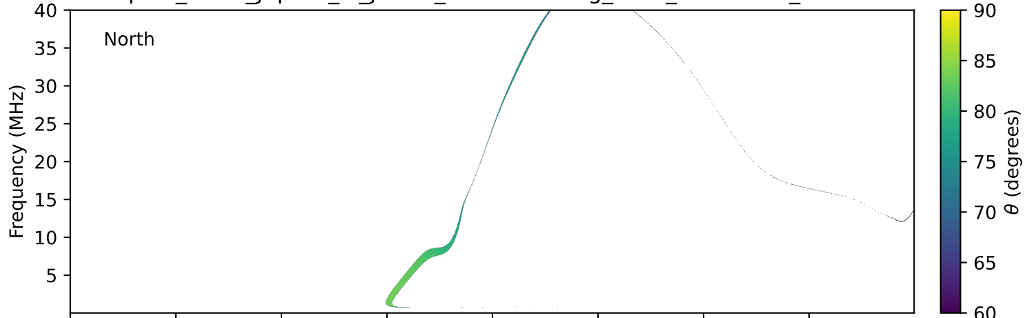
expres_earth_jupiter_io_jrm09_lossc-wid1deg_3kev_20030428_v11.cdf
