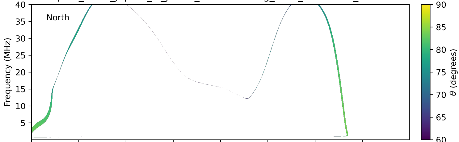
expres_earth_jupiter_io_jrm09_lossc-wid1deg_3kev_20030416_v11.cdf
