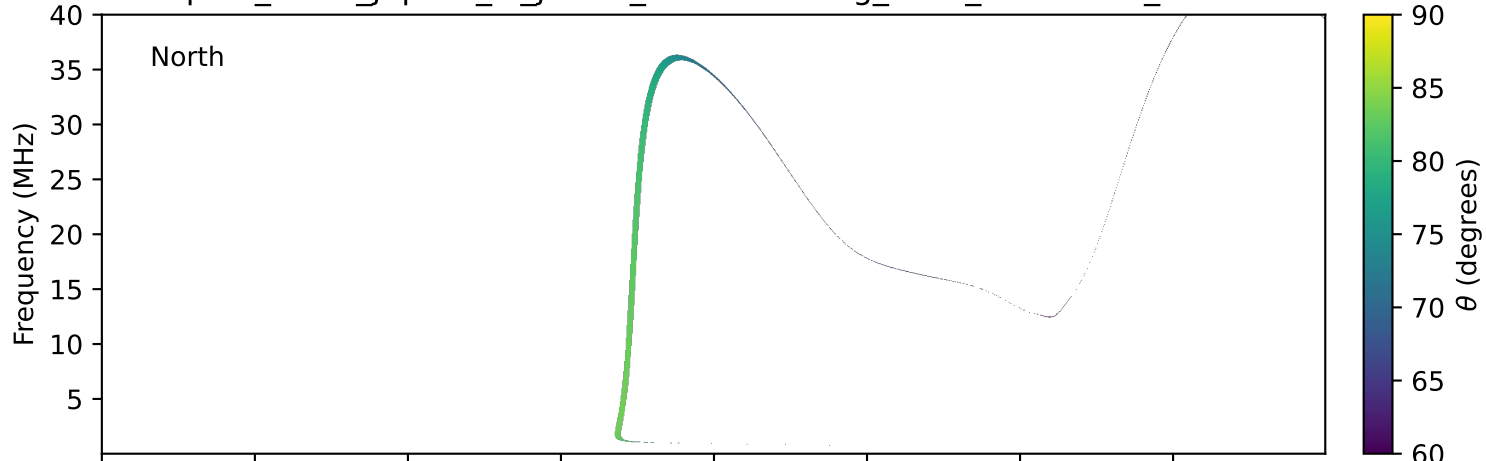
expres_earth_jupiter_io_jrm09_lossc-wid1deg_3kev_20030405_v11.cdf
