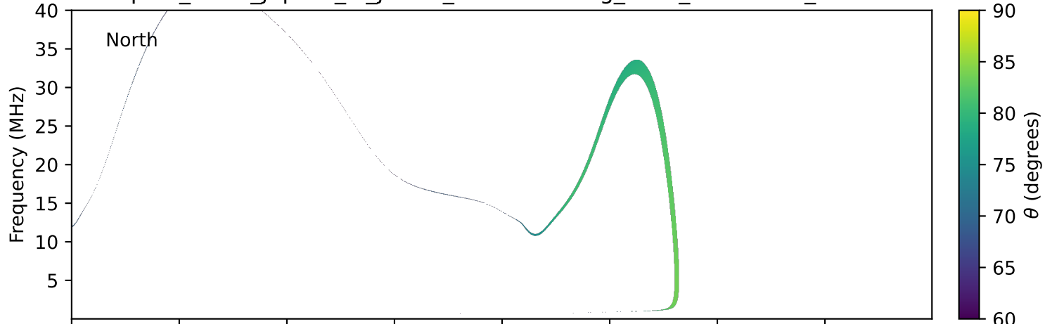
expres_earth_jupiter_io_jrm09_lossc-wid1deg_3kev_20030402_v11.cdf
