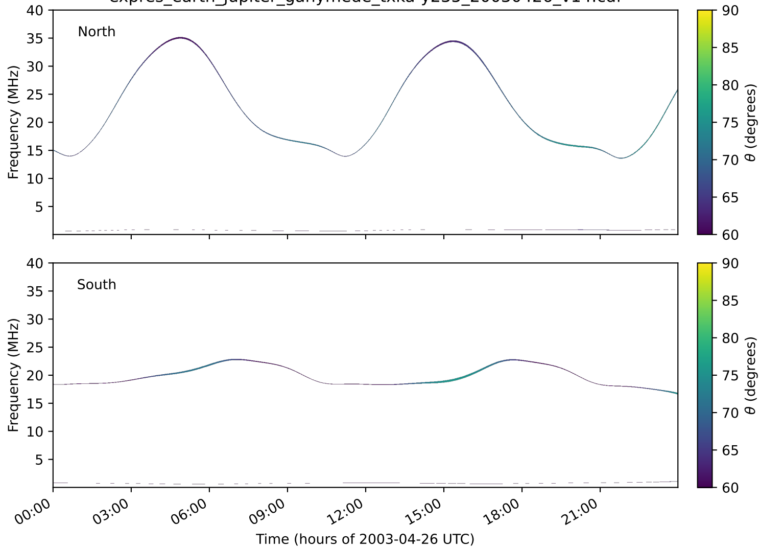
expres_earth_jupiter_ganymede_txka-y235_20030426_v14.cdf
