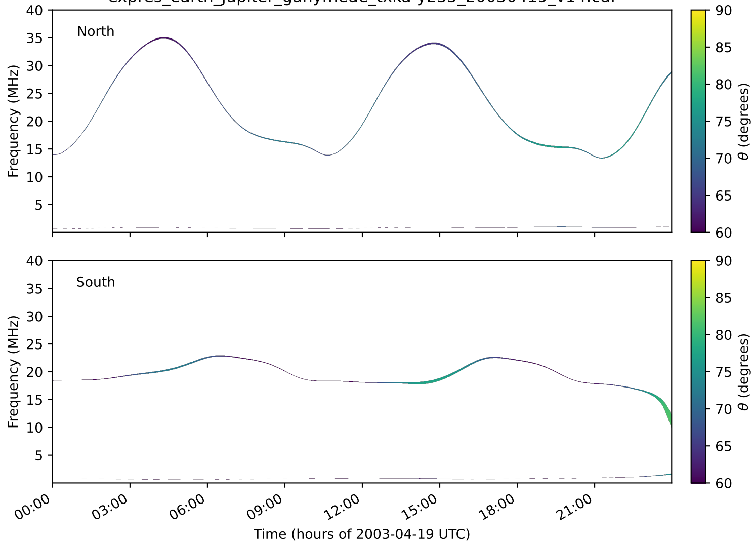
expres_earth_jupiter_ganymede_txka-y235_20030419_v14.cdf
