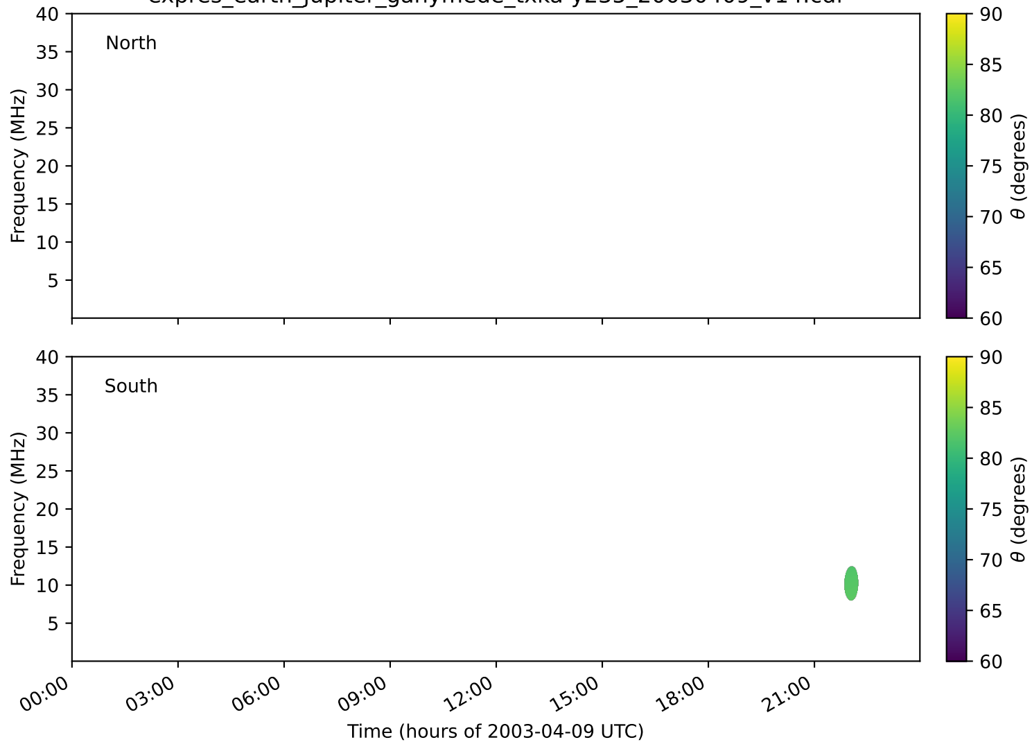
expres_earth_jupiter_ganymede_txka-y235_20030409_v14.cdf
