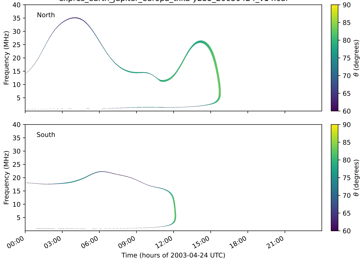
expres_earth_jupiter_europa_txka-y235_20030424_v14.cdf
