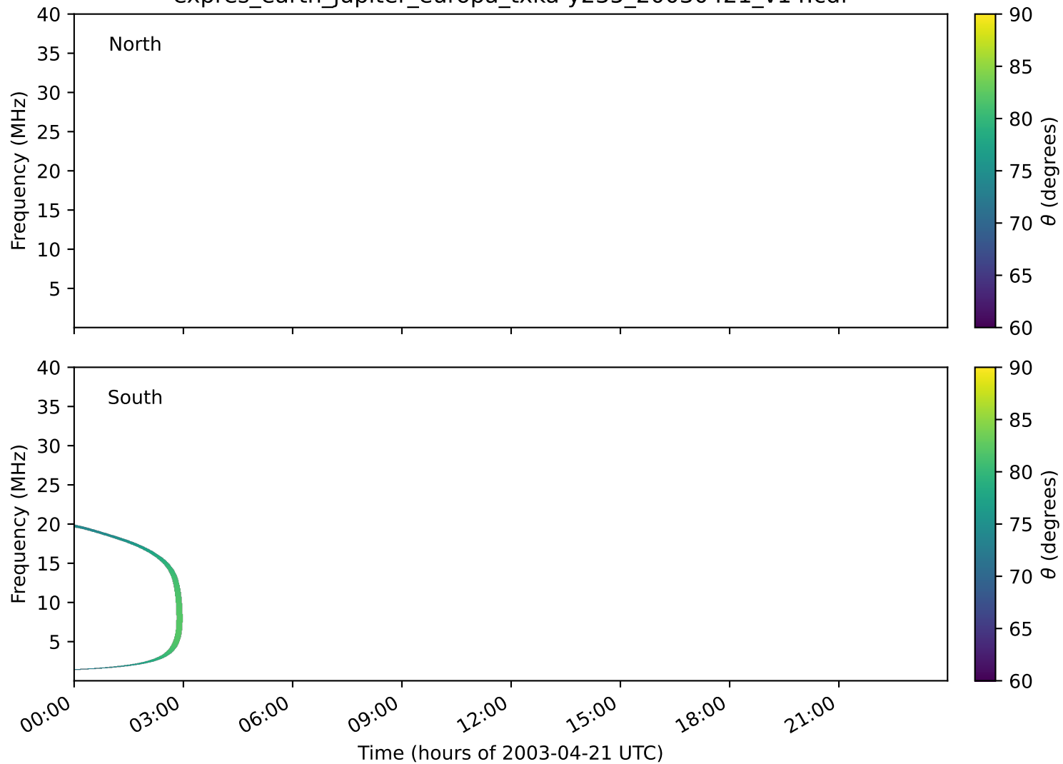
expres_earth_jupiter_europa_txka-y235_20030421_v14.cdf
