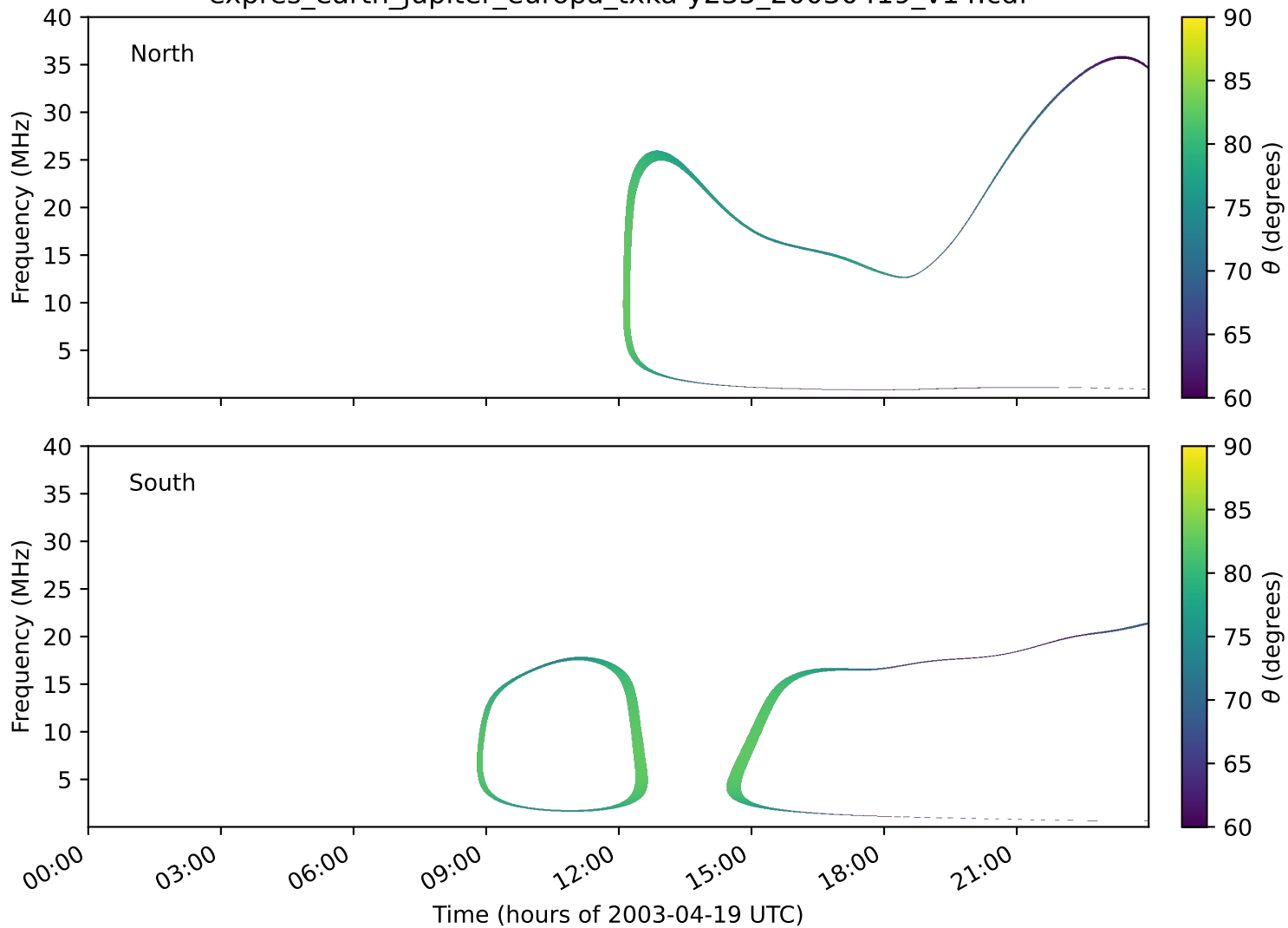
expres_earth_jupiter_europa_txka-y235_20030419_v14.cdf
